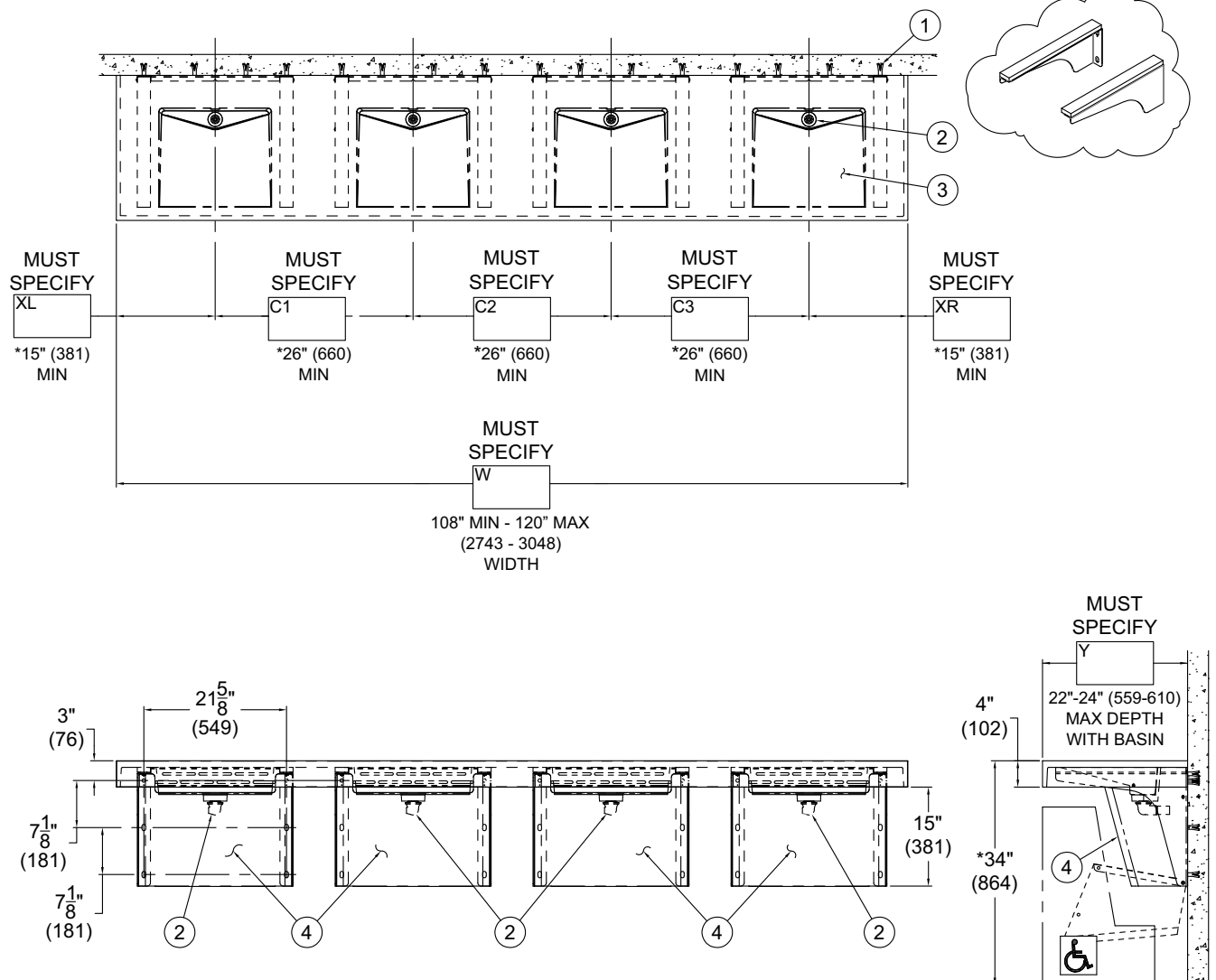
9220-4 SHOWN WITH FRONT MOUNT HINGED P-TRAP ENCLOSURE & EDGE BASIN
