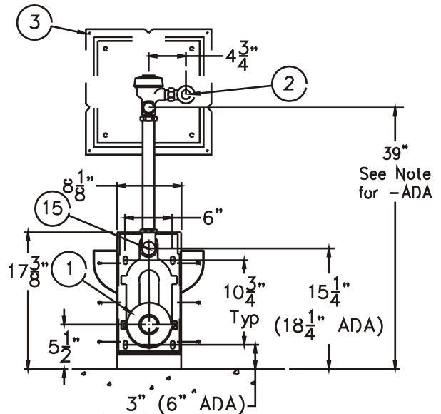
(-W) WALL SUPPLY VIEW FROM BACK OF FIXTURE
